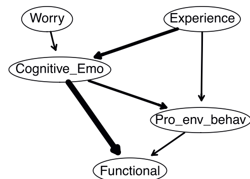
Fig. 4. Directed acyclic graphs (DAGs) With Arrow Thickness Denoting the Importance of that Arrow to the Overall Network Model Fit. Note. Arrow thickness denotes the importance of that arrow to the overall network model fit. Greater thickness reflects larger contribution to the model fit (i.e., Bayesian Information Criterion). Cognitive_emo = The cognitive-emotional component of climate anxiety; Functional = The functional component of climate anxiety; Pro_env_behav = Pro-environmental behaviors; Experience = Experience of climate change; Worry = General worry.
